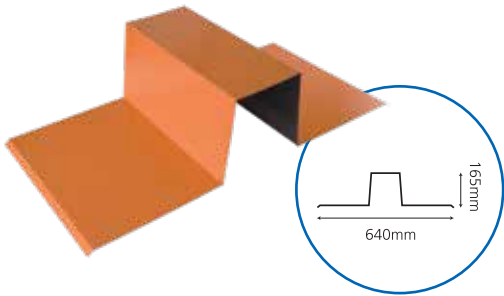
Valley Gutter
