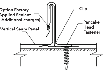
Vertical Seam Attachment Detail
