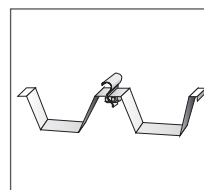
TH R505 standing seam roof connector
