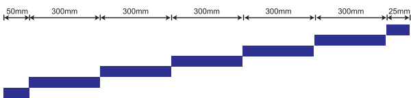
Roof Battens
