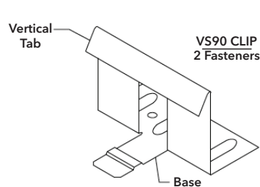
Vertical Seam Panel Clip
