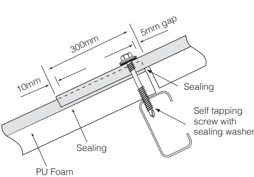
Panel End Lap
