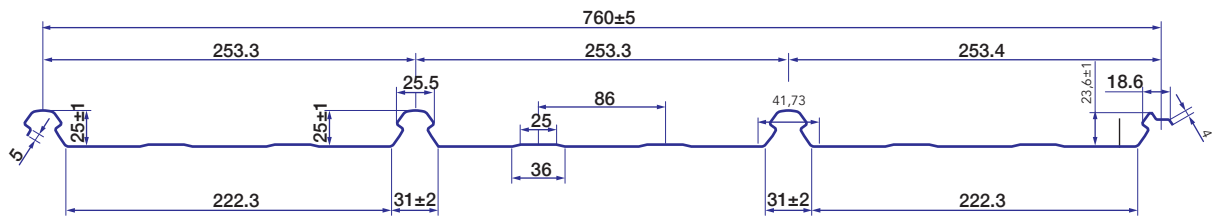
760 (Effective cover width) (All dimensions are in mm)
