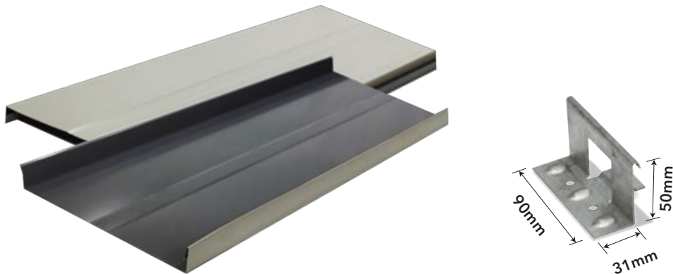
Vertical Seam Attachment Detail
