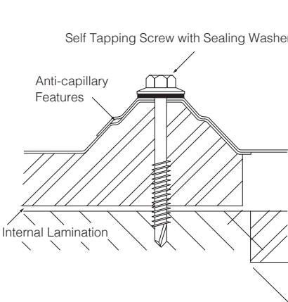
Panel End Lap
