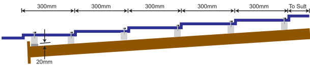
Roof Battens
