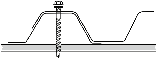
Crest fixing for roof or walls
