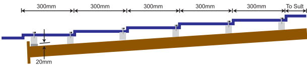
Roof Battens
