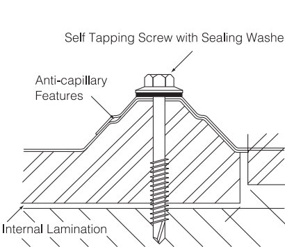
Panel End Lap
