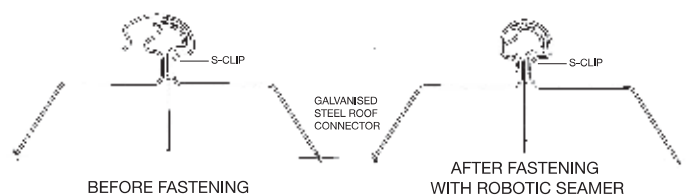
Side Lap
