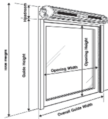
How to Measure Shutter Door Dimension:
