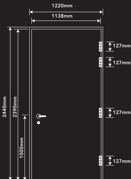
Door Frame Size - Single Leaf (maximum size 1220mm x 2440mm)
